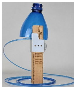
Figura 5. Plastic Bottle Cutter
