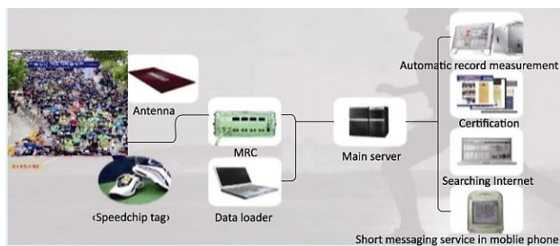
Figura 10. Timing system configuration and application [10]
