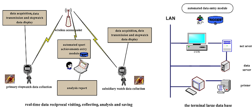
Figura 9. System Architecture [9]
