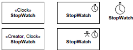
Figure 12.25 Presentation Options for an Extended Class
