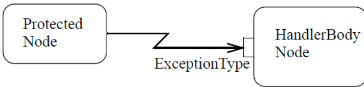
Figure 15.62 ExceptionHandler notation
