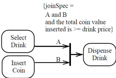
Figure 15.38 joinSpec example
