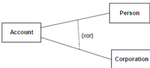
Figure 7.16 {xor} constraint
