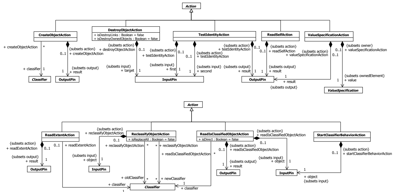
Figure 16.30 Object Actions
