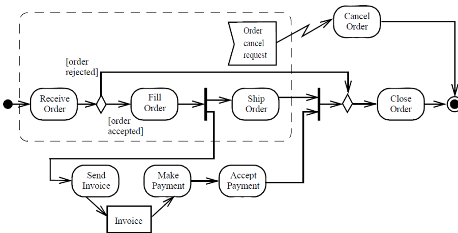
Figure 15.73 InterruptibleActivityRegion example
