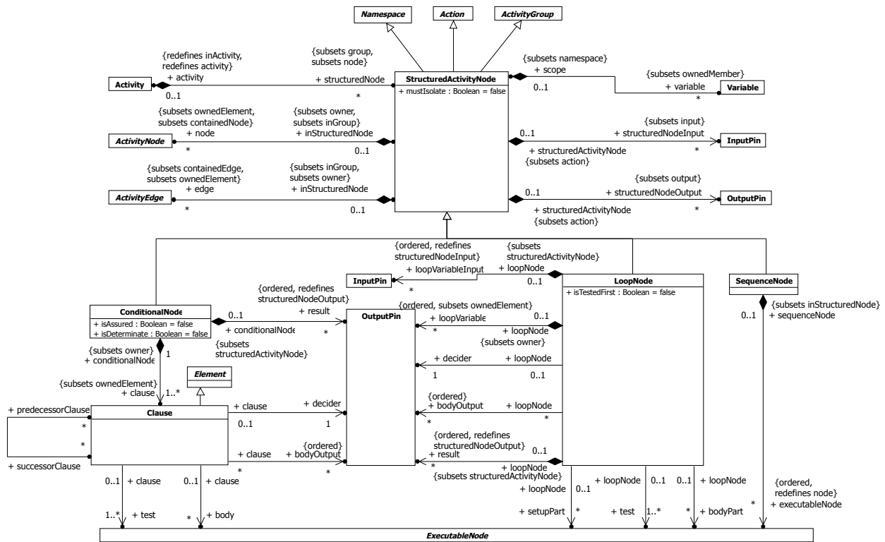
Figure 16.45 Structured Actions
