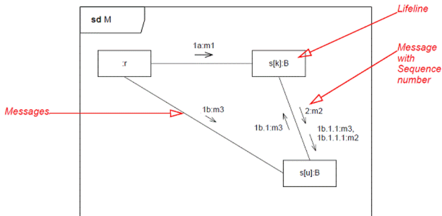
Figure 17.26 Communication diagram
