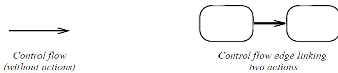
Figure 15.8 ControlFlow notation
