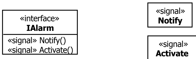
Figure 10.6 Reception Notation
