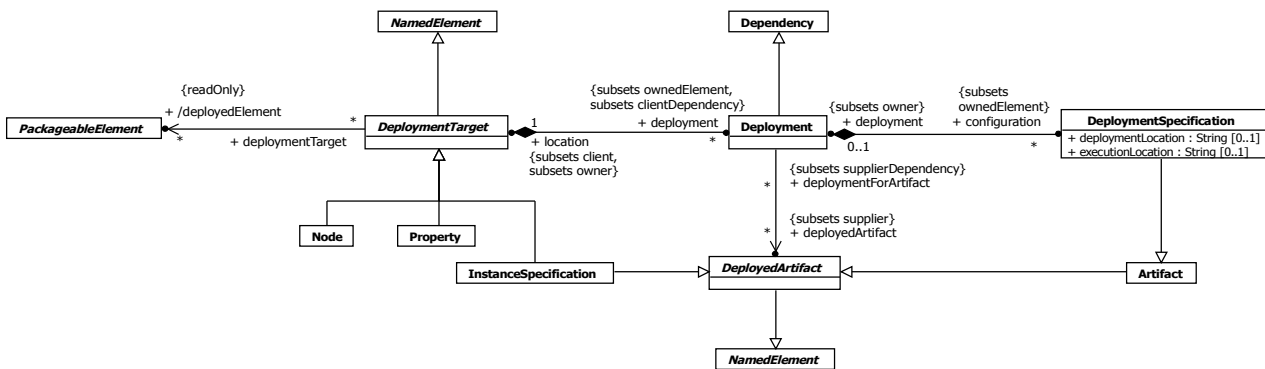
Figure 19.1 Deployments
