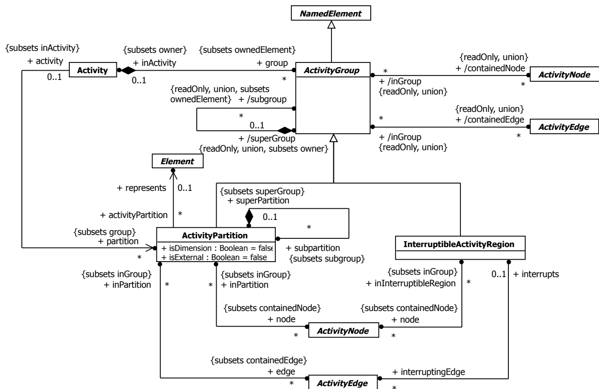
Figure 15.65 ActivityGroups
