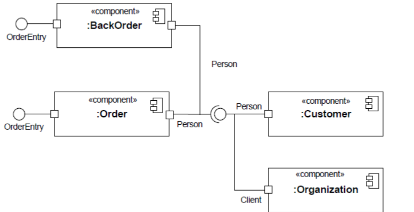
Figure 11.9 An n-ary Connector that assembles four simple Ports using channeled ball-and-socket notation.
