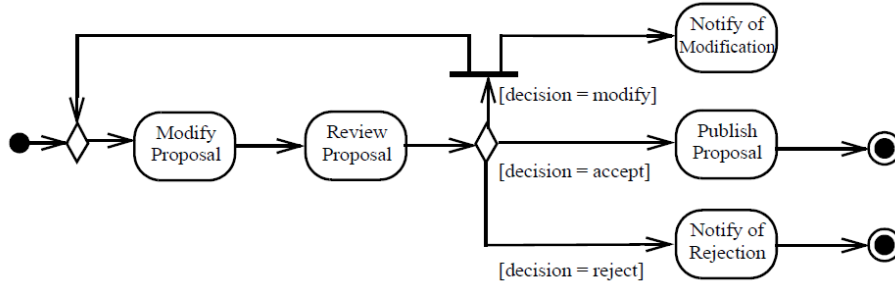
Figure 15.44 ActivityFinalNode example
