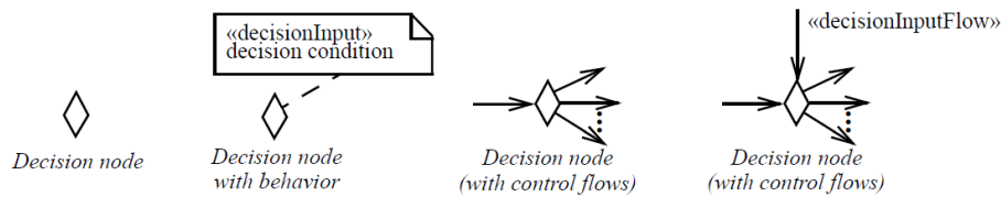
Figure 15.33 DecisionNode notation
