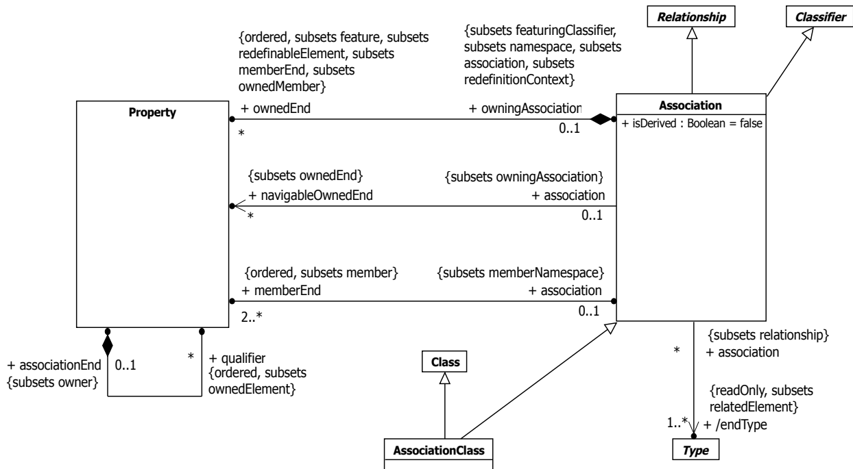
Figure 11.25 Associations
