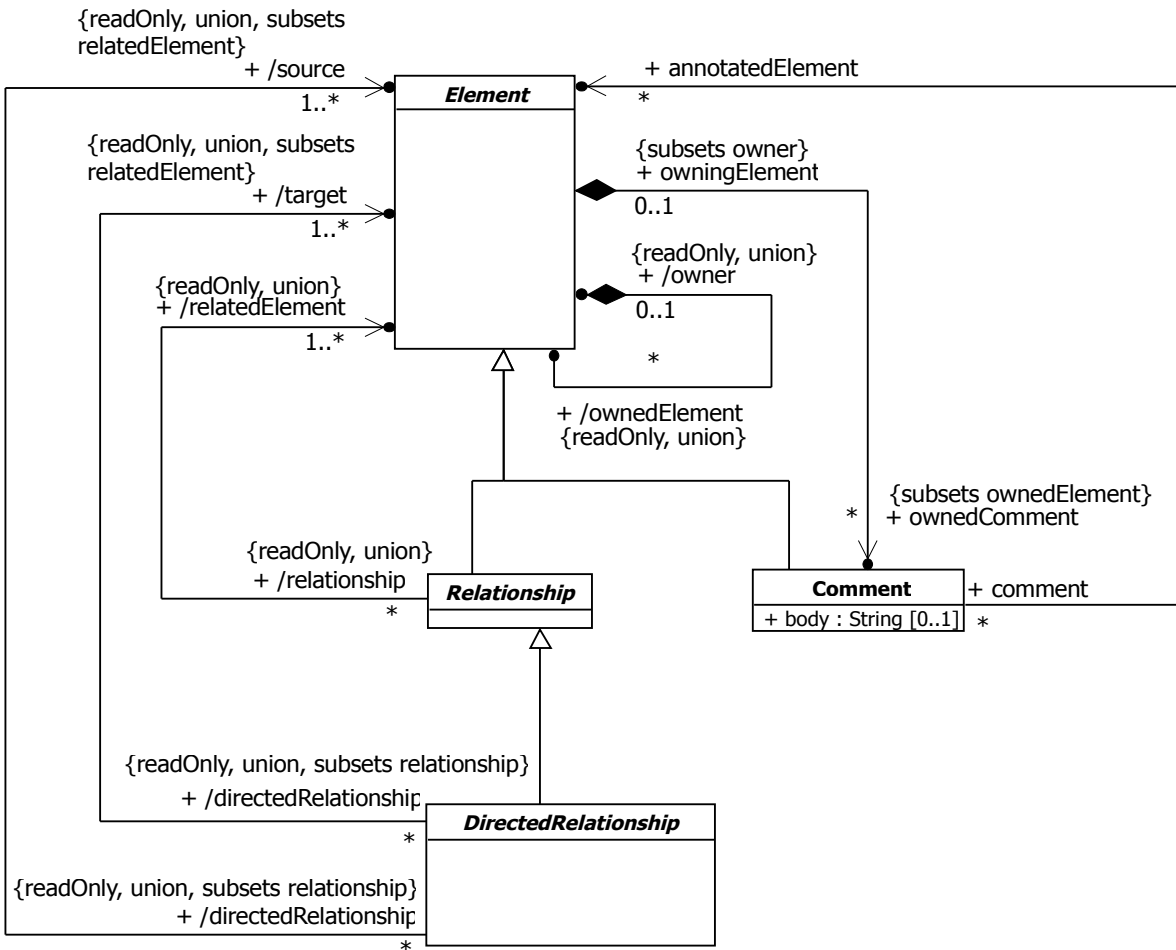
Figure 7.1 Root
