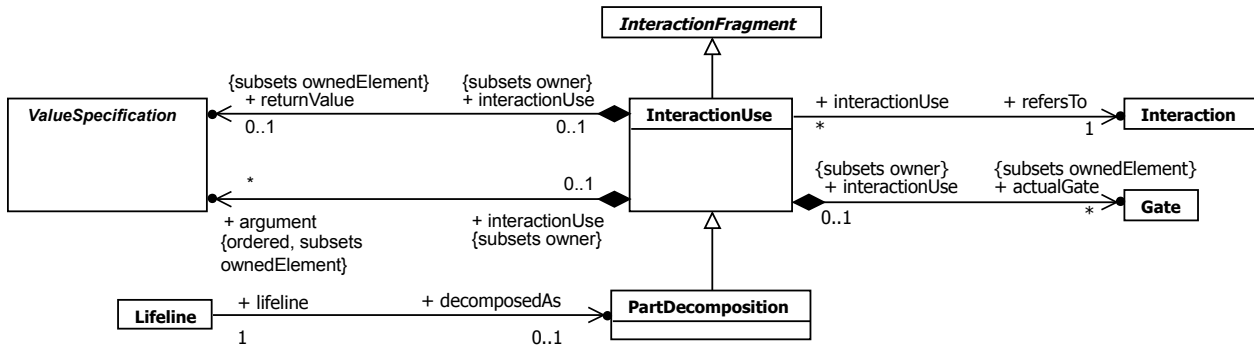
Figure 17.18 InteractionUses
